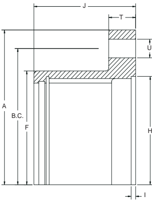
(FLANGED SLEEVE AND RIGID HUB DETAILS)
